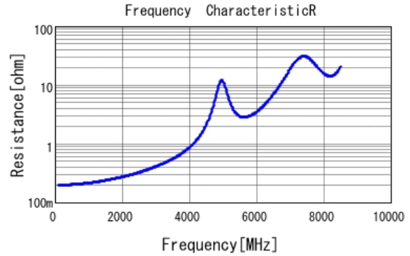
■ GCM1885C2A9R0CA16 R DCOV, 25degC
