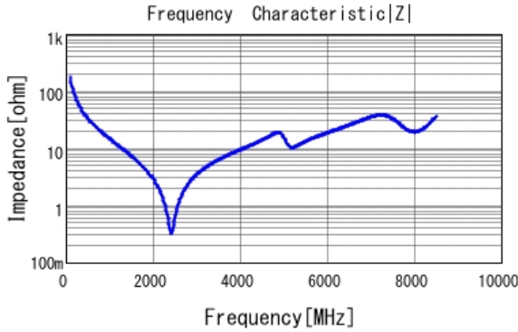
■ GCM1885C2A9R0CA16 |Z| DCOV, 25degC
