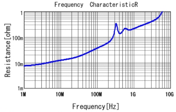
GCM1885C1K362GA16 R DCOV, 25degC
