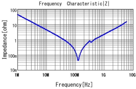
GCM1885C1K362GA16 |Z| DCOV, 25degC
