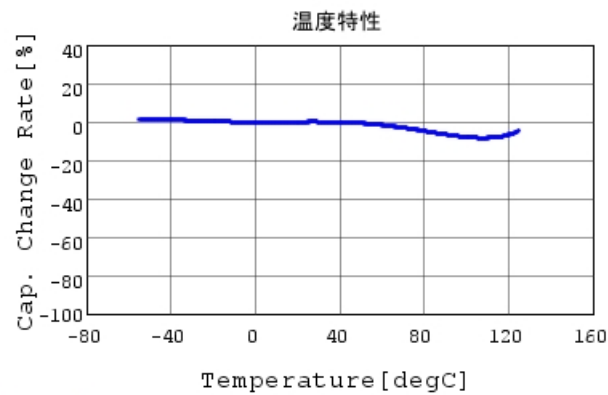
GCM155R71H681KA37 C-Temp. capchange, DC0.0V,
