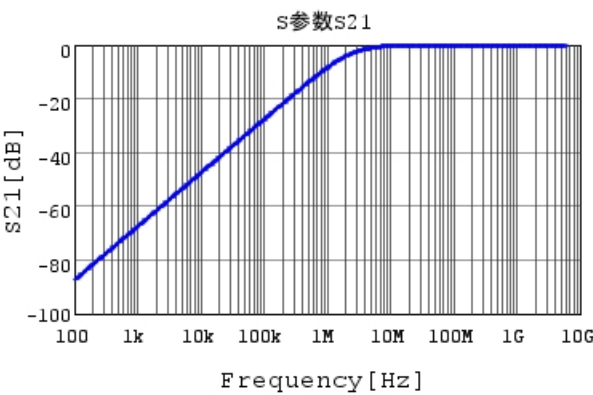
GCM155R71H681KA37 S21 DC0V, 25degC
