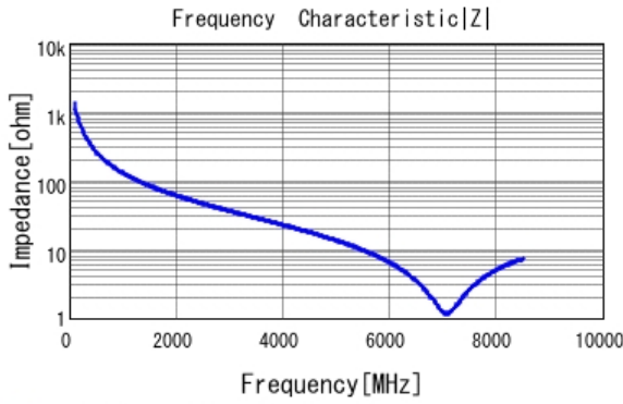
■ GCM1555C1H1R2BA16 |Z| DC0V, 25degC
