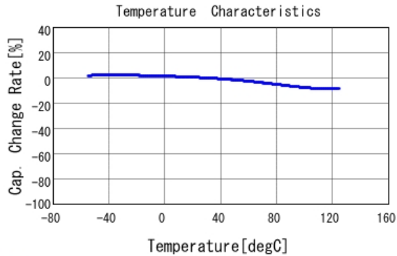
■ GCM033R71C222KA55 C-Temp. capchange, DC0.0V, AC1.0V rm
