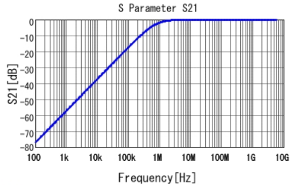
■ GCM033R71C222KA55 S21 DC0V, 25degC
