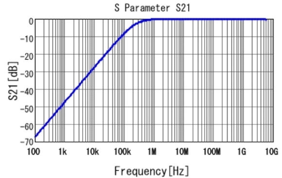
■ GCJ188R72A682KA01 S21 DC0V, 25degC
