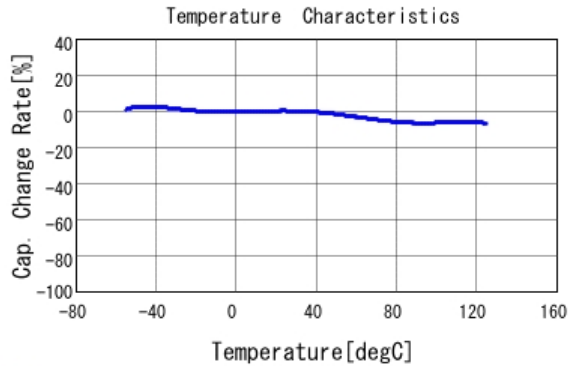
■ GCJ188R72A682KA01 C-Temp. capchange, DC0.0V, AC1.0V rm
