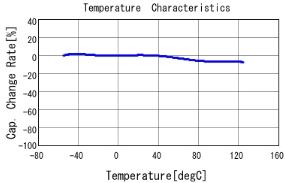
■ GCJ188R72A332KA01 C-Temp. capchange, DC0.0V, AC1.0V rm
