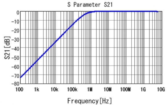
■ GCJ188R72A332KA01 S21 DC0V, 25degC
