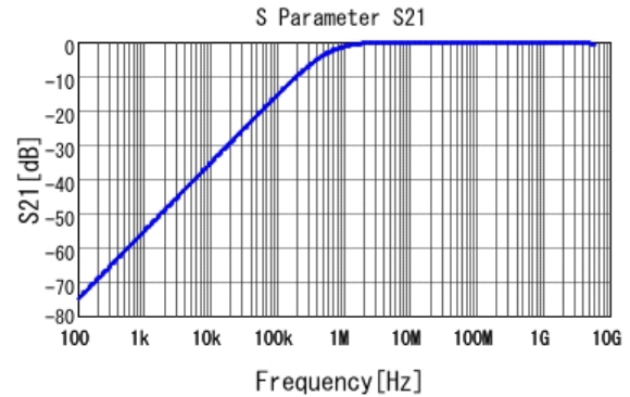
■ GCJ188R71H272KA01 S21 DC0V, 25degC
