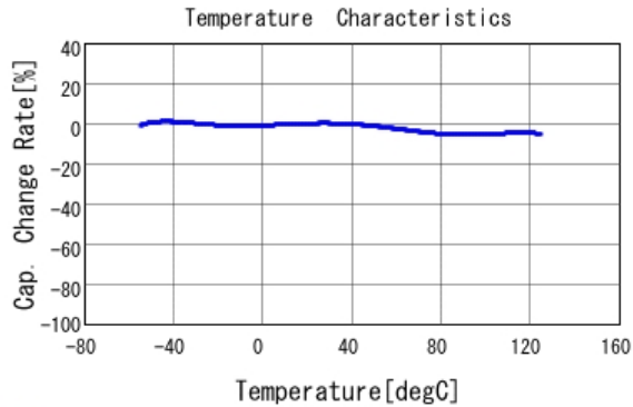
■ GCJ188R71H272KA01 C-Temp. capchange, DC0.0V, AC1.0V rm
