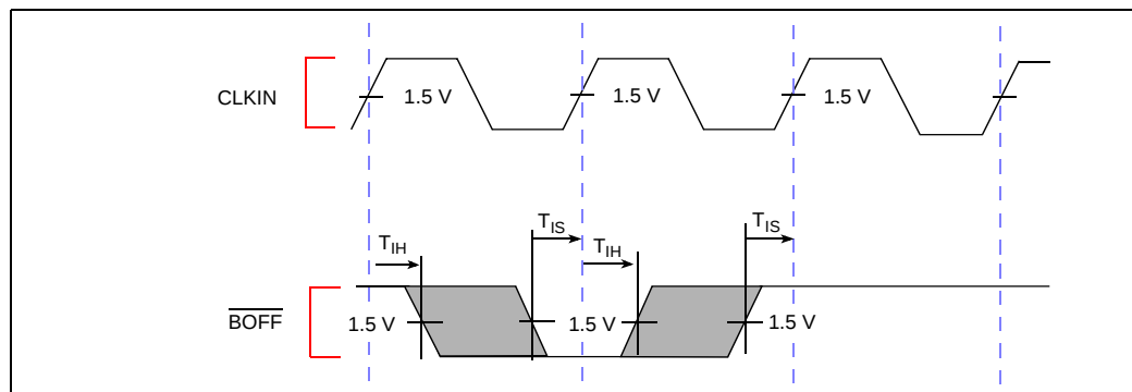
Figure 16. Bus Backoff ( \overline{\text{BOFF}} ) Timings
