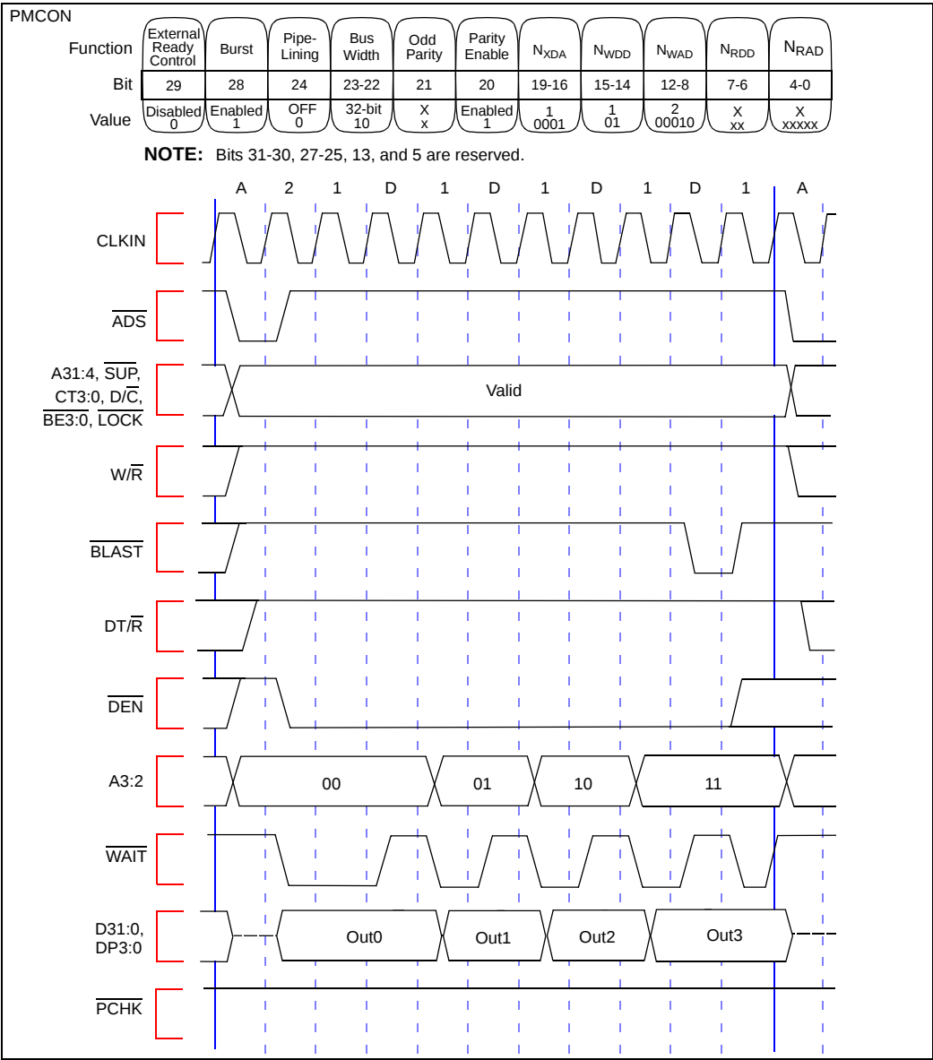
Figure 38. Burst, Non-Pipelined Write Request with Wait States, 32-Bit Bus
