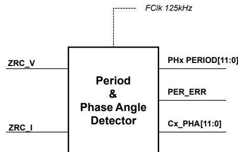
Figure 41. Phase meter
