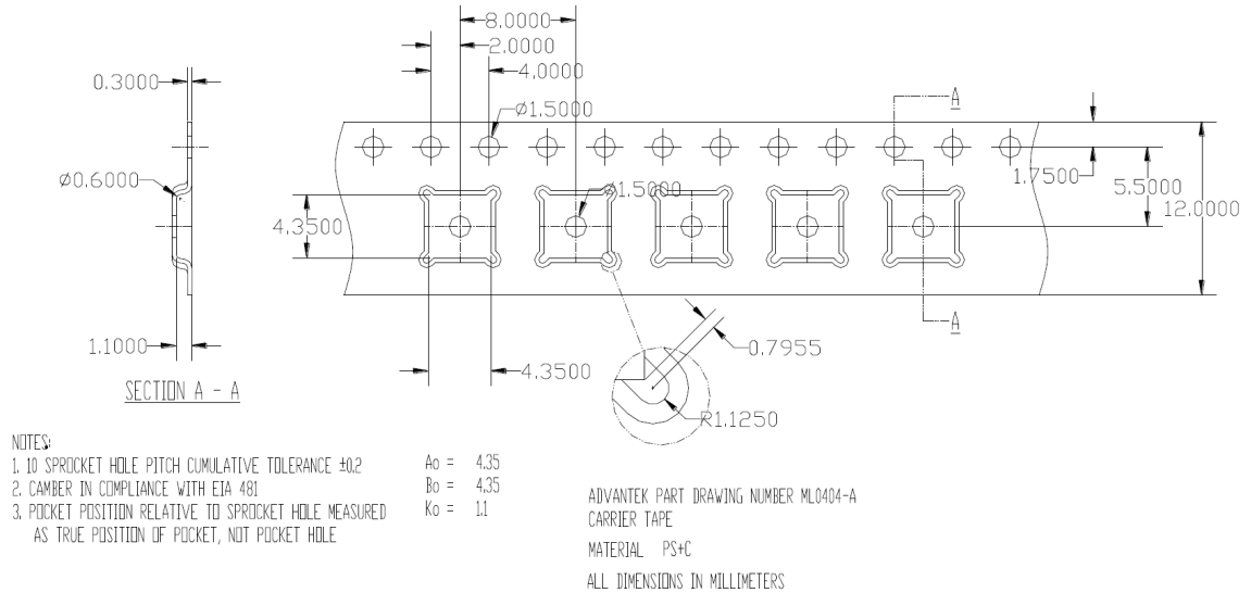
Figure 63. QFN24L (4x4x1) carrier tape outline
