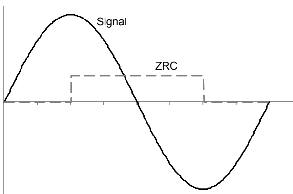
Figure 40. Zero-crossing signal
