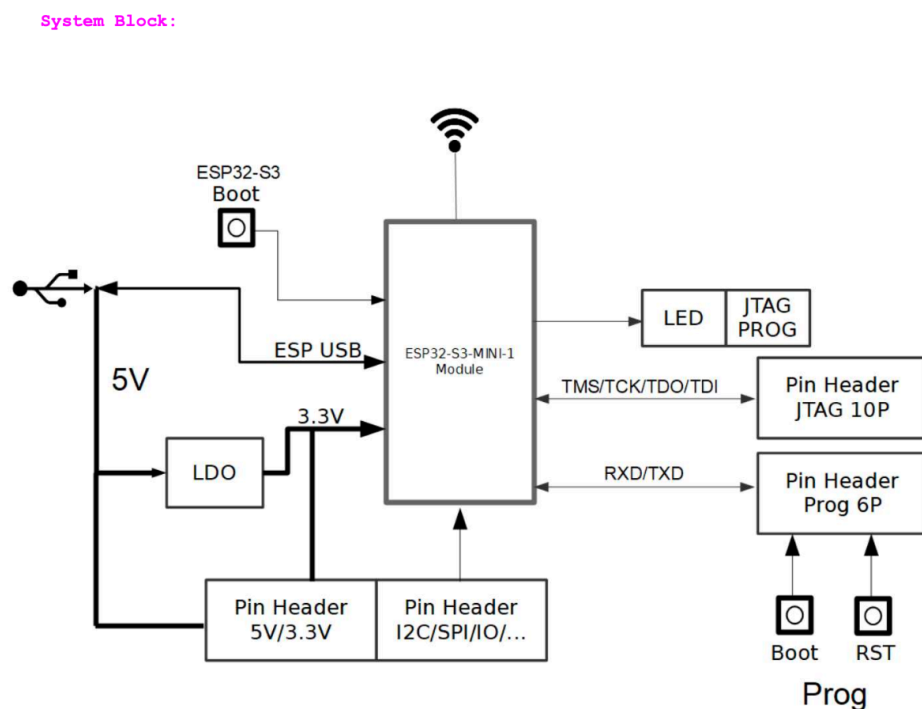
Fig. 4: ESP-Prog-2 Block Diagram (click to enlarge)
