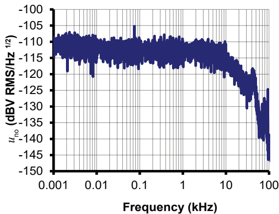
Figure 13: Typical noise voltage spectral density u_{no} with R_M = 50 \Omega
