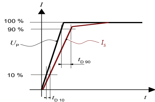
Figure 17: Delay time t_{D90} @ 90 and delay time t_{D10} @ 10
