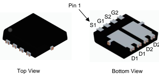
POWERDI®3333-8/SWP (Type UXD)
