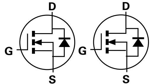
Internal Schematic
