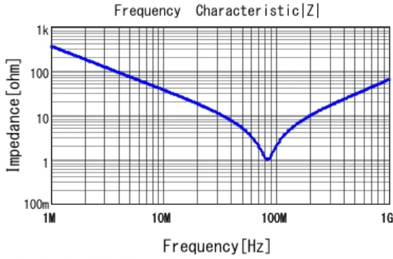
■ DE2B3SA471KJ3BT02F |Z| DCOV, 20degC
