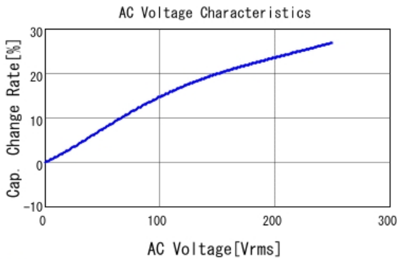
■ DE2B3SA471KJ3BT02F C-AC Voltage capchange, DCOV, 20.0
