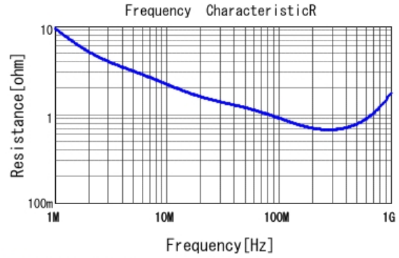
■ DE2B3SA471KJ3BT02F R DCOV, 20degC
