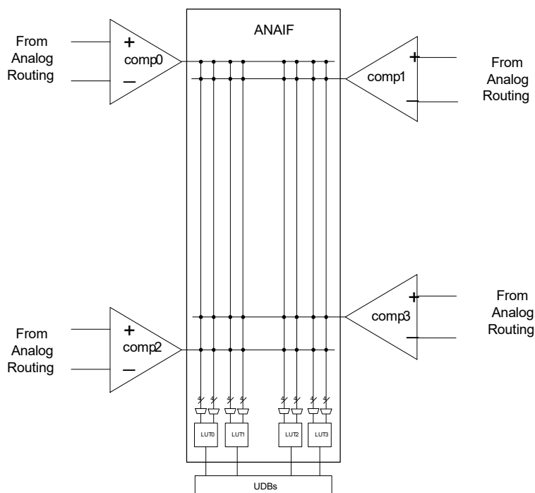
Figure 8-5. Analog Comparator
