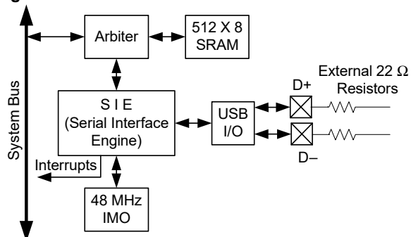
Figure 7-16. USB
