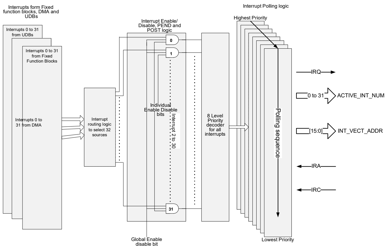
Figure 4-3. Interrupt Structure
