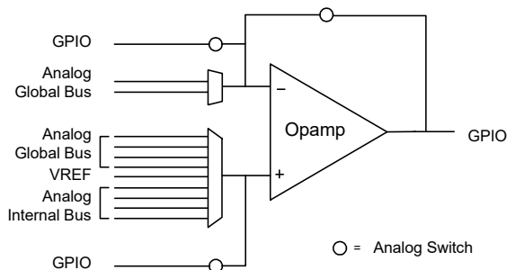
Figure 8-6. Opamp
