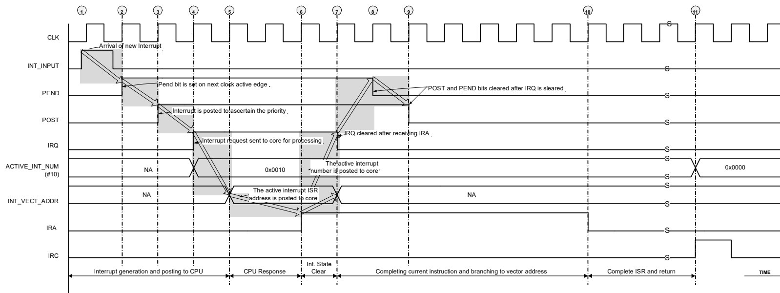
Figure 4-2. Interrupt Processing Timing Diagram
