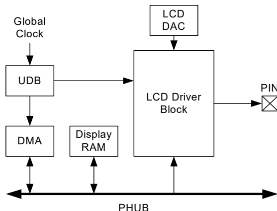
Figure 8-10. LCD System
