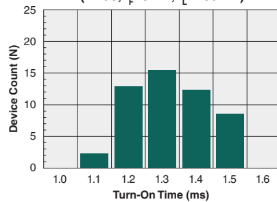
Typical Turn-On Time (N=50, I_F=3\text{mA} , I_L=100\text{mA} )
