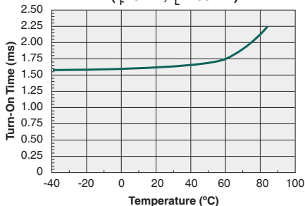
Typical Turn-On Time vs. Temperature ( I_F=3\text{mA} , I_L=100\text{mA} )
