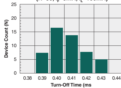
Typical Turn-Off Time (N=50, I_F=3\text{mA} , I_L=100\text{mA} )
