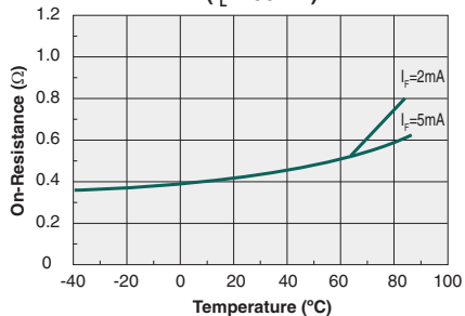
Typical On-Resistance vs. Temperature ( I_L=100\text{mA} )
