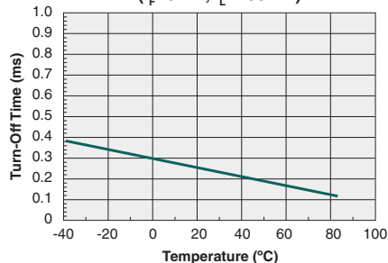
Typical Turn-Off Time vs. Temperature ( I_F=3\text{mA} , I_L=100\text{mA} )
