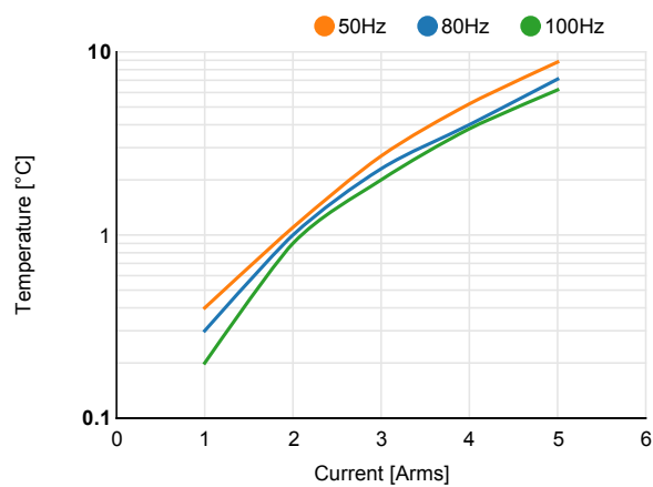
Ripple Current
