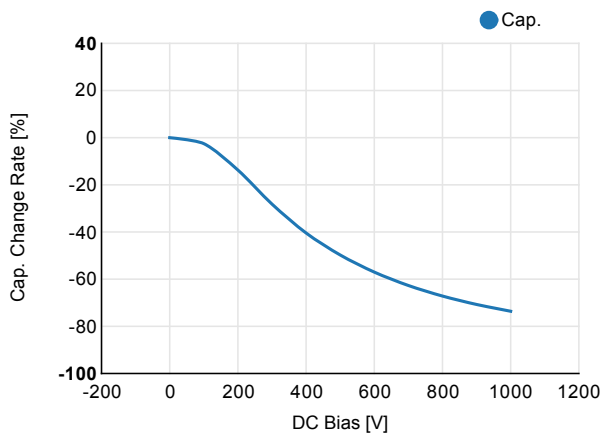
DC Bias
