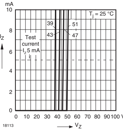
Figure 18. Breakdown Characteristics
