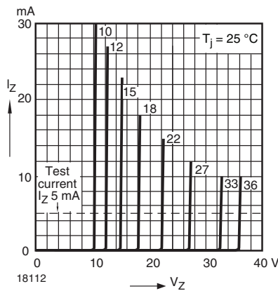
Figure 17. Breakdown Characteristics
