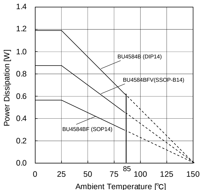
Figure 11. Derating Curve
