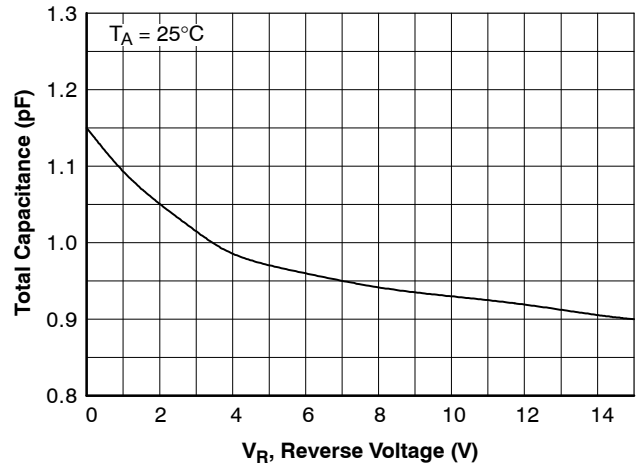
Figure 8. Total Capacitance
