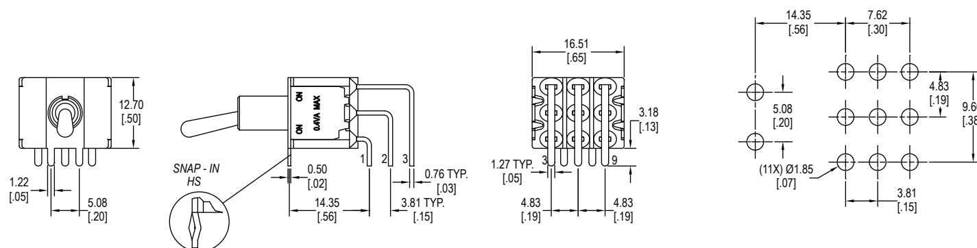
V (VS - Snap-in) = Vertical mount, right angle PC pins, three pole
