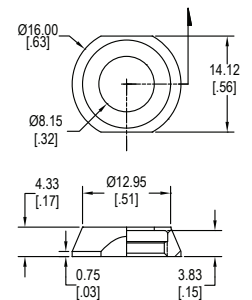
Dress Nut
