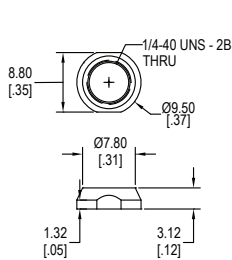
Dress Nut C
