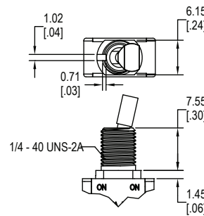
AR1 - Threaded Anti-Rotation
