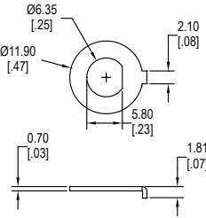
Locking Ring-Flat
