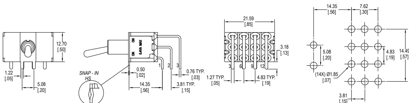
V (VS - Snap-in) = Vertical mount, right angle PC pins, four pole
