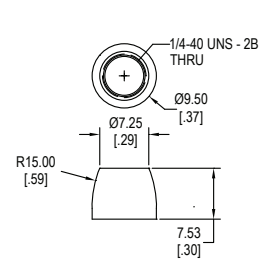
Dress Nut E
