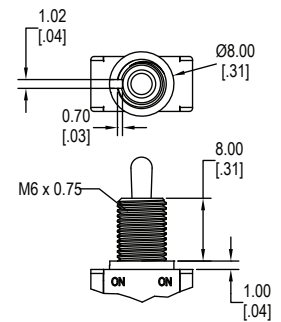
W - Threaded Metric
