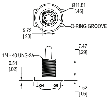
L - Threaded Splash Proof
