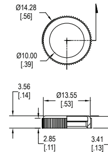
Knurled Nut
