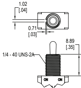
E - Threaded E1 - Non-Treaded
