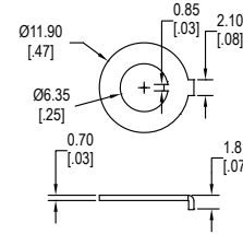
Locking Ring-Keyway
