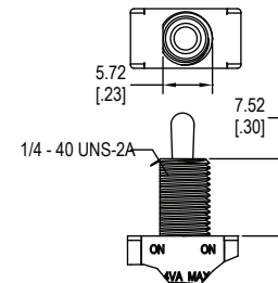
G - Threaded High Torque
