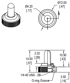
Sealed Boot E Knurled Nut
