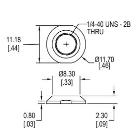
Dress Nut D
