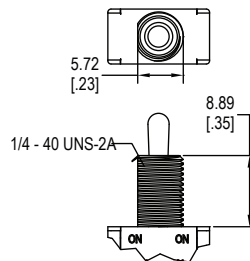
J - Threaded
