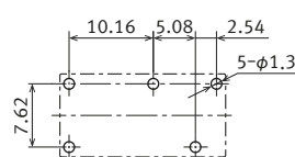
Recommended PC board pattern ( BOTTOM VIEW )
