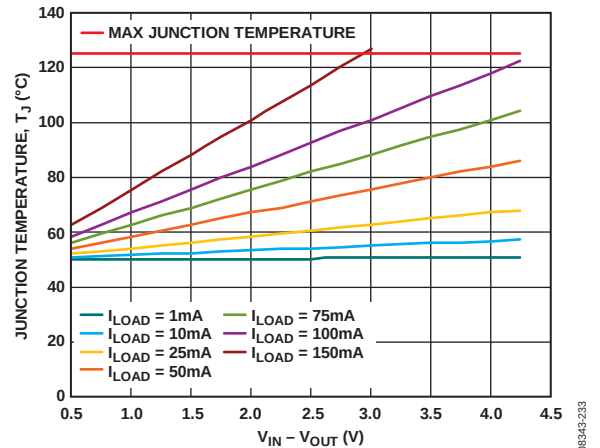
Figure 38. TSOT, 0 mm 2 of PCB Copper, T_A = 50^{\circ}\text{C}
