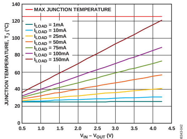
Figure 40. WLCSF, 500 mm 2 of PCB Copper, T_A = 25^{\circ}\text{C}
