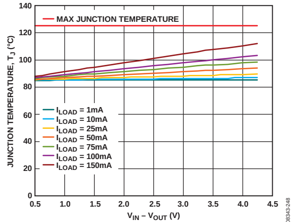
Figure 39. TSOT, 100 mm 2 of PCB Copper, Board Temperature = 85 ^{\circ}\text{C}
