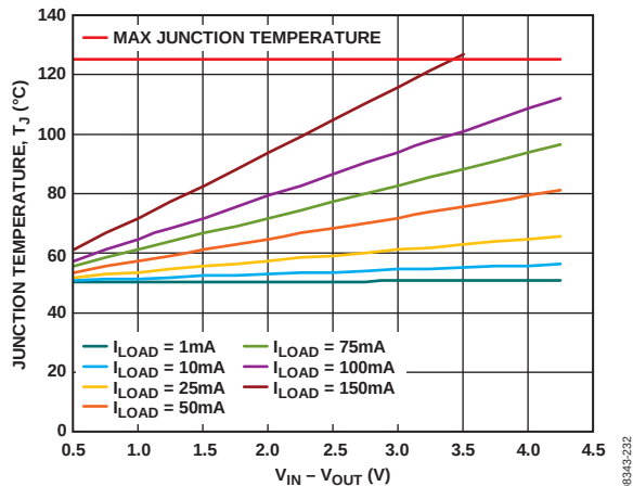
Figure 37. TSOT, 100 mm 2 of PCB Copper, T_A = 50^{\circ}\text{C}
