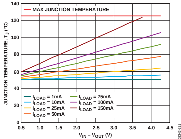
Figure 36. TSOT, 500 mm 2 of PCB Copper, T_A = 50^{\circ}\text{C}
