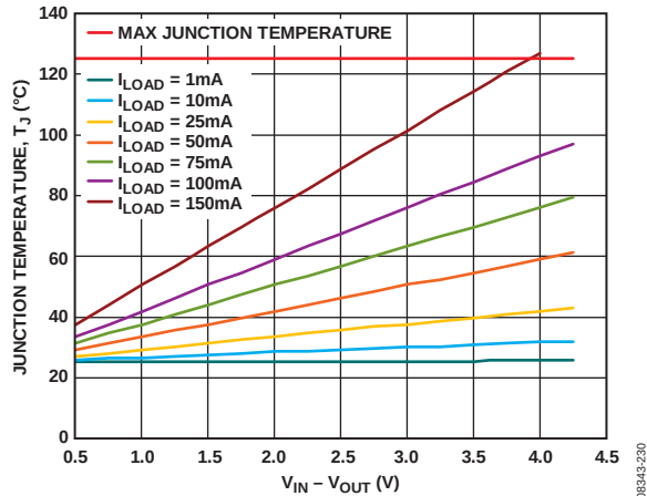
Figure 35. TSOT, 0 mm 2 of PCB Copper, T_A = 25^{\circ}\text{C}
