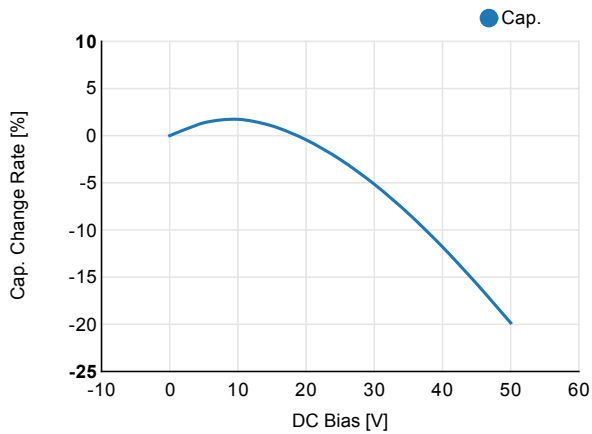
DC Bias
