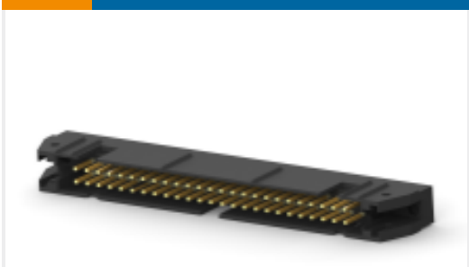
TE Part # 5499160-8 AMP-LATCH UNIVERSAL HEADERS
