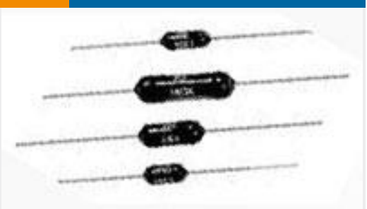
TE Part # 1879660-9 H4 15K 0.1% 15PPM
