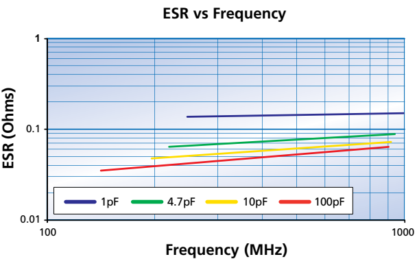
Typical performance data - 1111 chip size*
