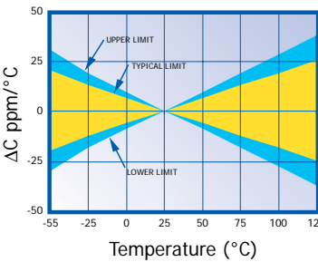
COG/NPO capacitance vs temperature
