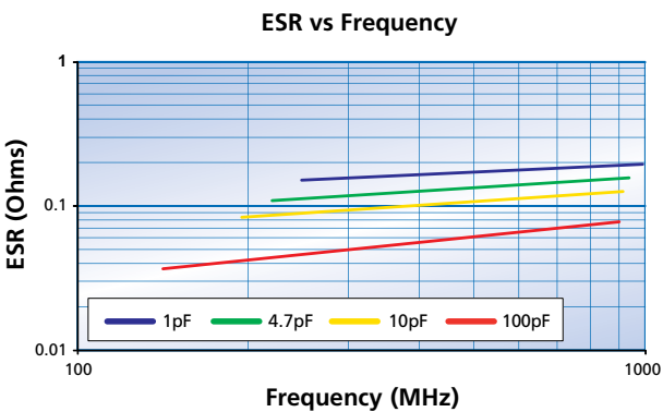
Typical performance data - 0805 chip size*
