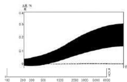
Long Term Stability BS CECC 40101 030 Ratings at 125°C H4 - 0.125 W
