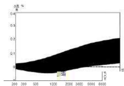
Long Term Stability BS CECC 40101 004 Ratings at 70°C H4 - 0.25 W H80
