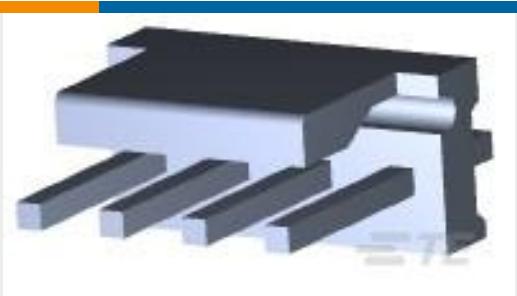
TE Part # 3-640441-3 MTA Receptacle: Nylon, Tin Plated, 2.54 mm
