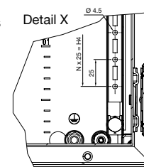
5 6 Pre-drilled holes for plinths/eyebolts only for specified sizes
