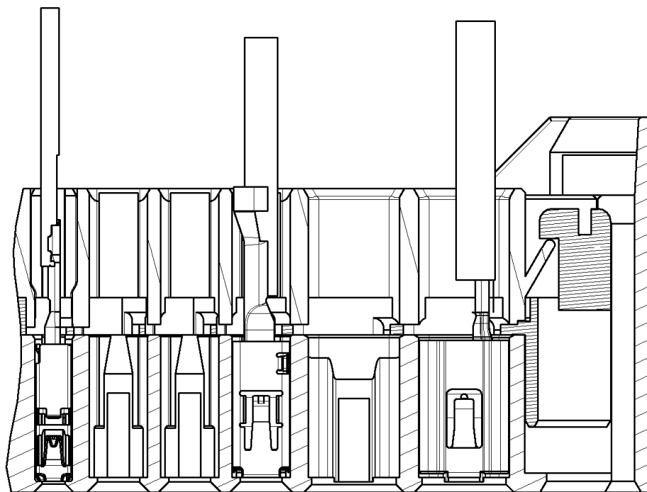
Retainer in end-locked position / Retainer in Endraststellung
