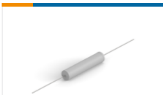
TE Part # 9-2176415-0 8W STD M/OX 5% 150K
