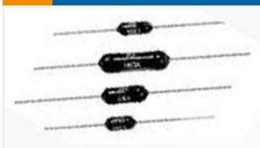
TE Part # 7-1879645-2 H8 301R 0.5% 50PPM
